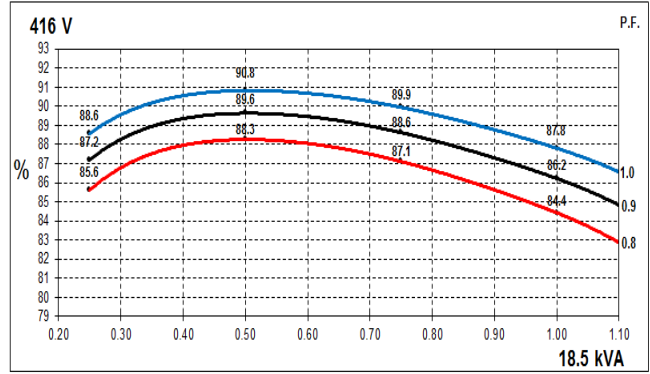
60Hz Curves
