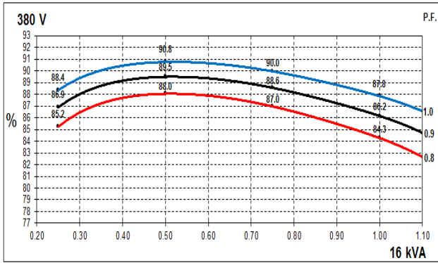
50Hz Curves
